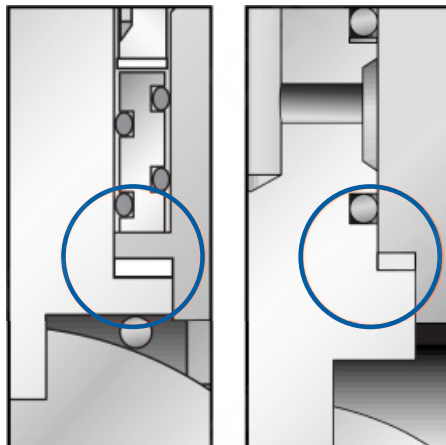
Class 150 & 300
